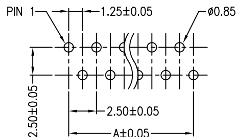
SPECIAL PCB LAYOUT
